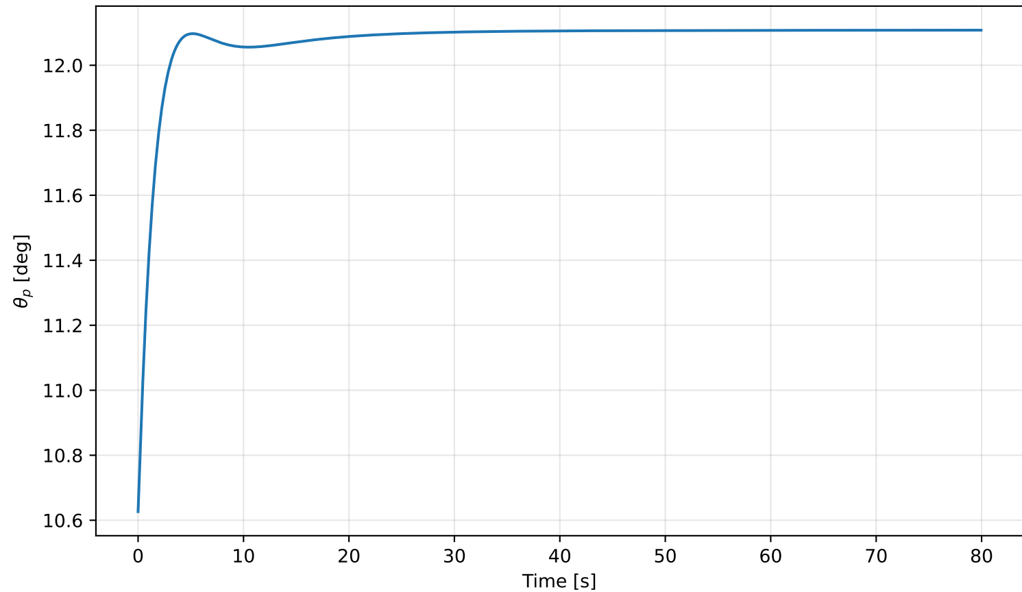
Above-rated pitch response at V_0 = 16.0 m/s
